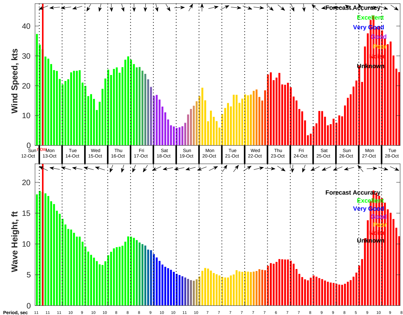
Wind & Wave Forecast for NDBC 44008 from 12-Oct-2025 20:00:00 to 28-Oct-2025 20:00:00
