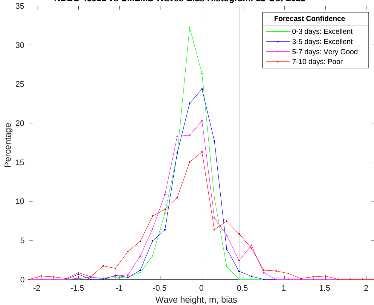
NDBC 46011 vs CMEMS Waves Bias Histogram: 13-Oct-2025
