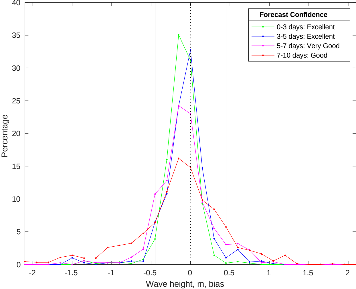
NDBC 46028 vs CMEMS Waves Bias Histogram: 13-Oct-2025
