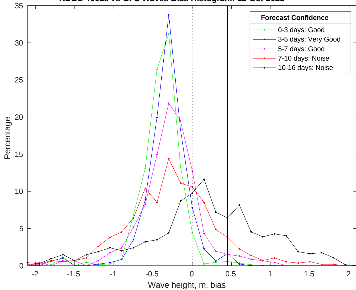
NDBC 46028 vs GFS Waves Bias Histogram: 13-Oct-2025
