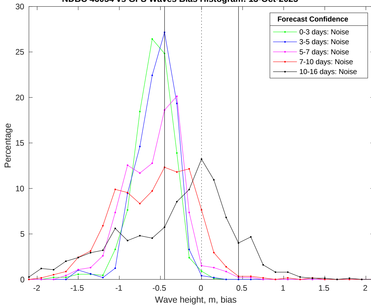
NDBC 46054 vs GFS Waves Bias Histogram: 13-Oct-2025
