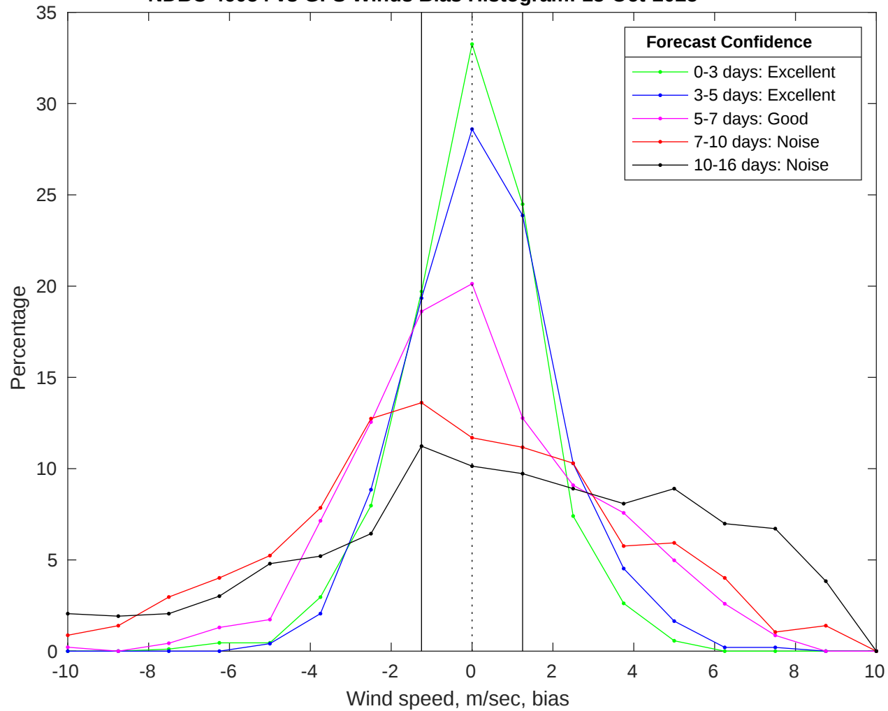
NDBC 46054 vs GFS Winds Bias Histogram: 13-Oct-2025
