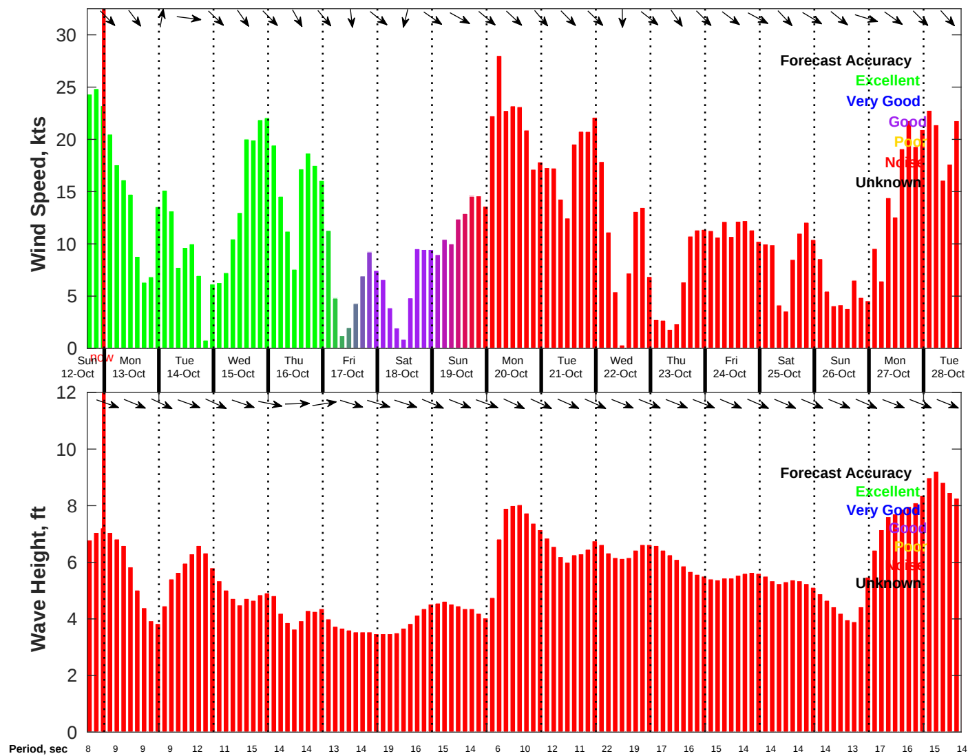
Wind & Wave Forecast for NDBC 46054 from 12-Oct-2025 16:00:00 to 28-Oct-2025 16:00:00
