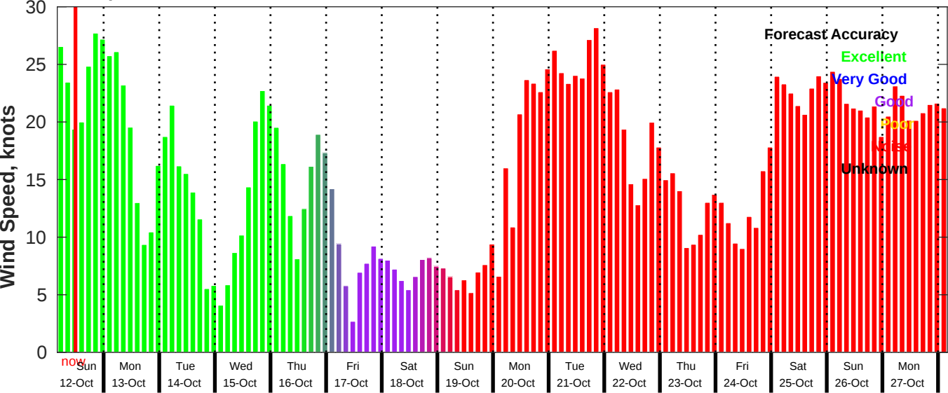
GFS Wind Speed Forecast for NDBC 46069 from 12-Oct-2025 04:00:00 to 28-Oct-2025 04:00:00
