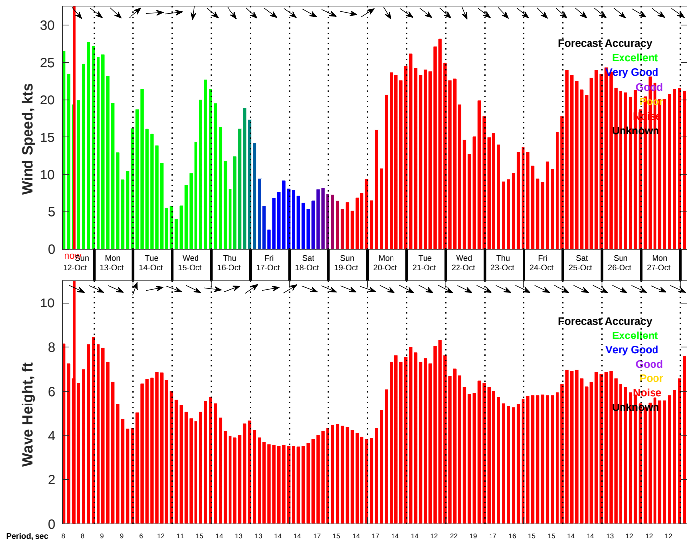
Wind & Wave Forecast for NDBC 46069 from 12-Oct-2025 04:00:00 to 28-Oct-2025 04:00:00
