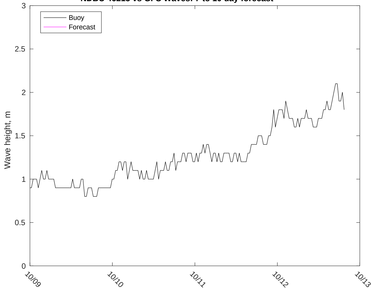
NDBC 46215 vs GFS Waves: 7 to 10 day forecast
