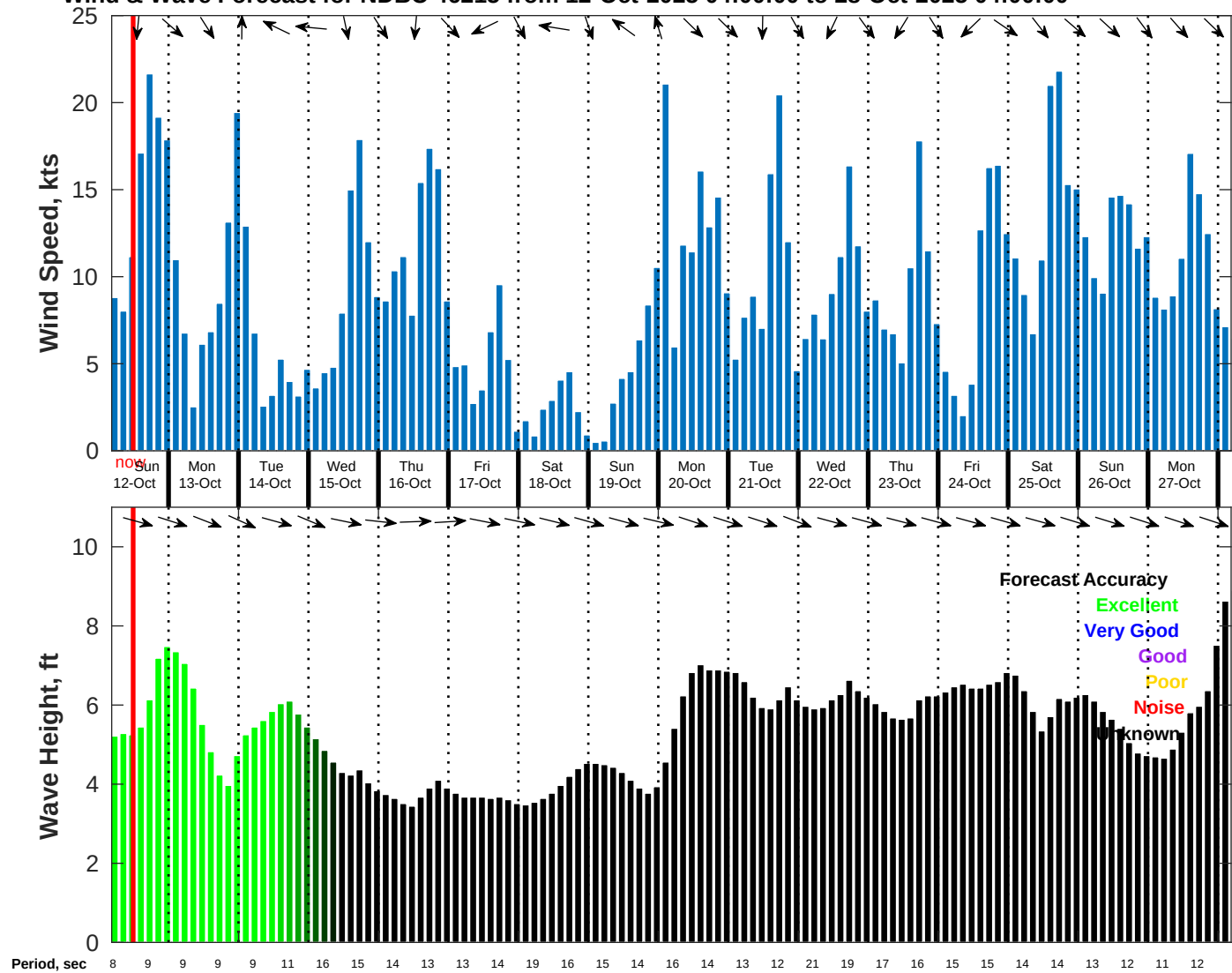
Wind & Wave Forecast for NDBC 46215 from 12-Oct-2025 04:00:00 to 28-Oct-2025 04:00:00
