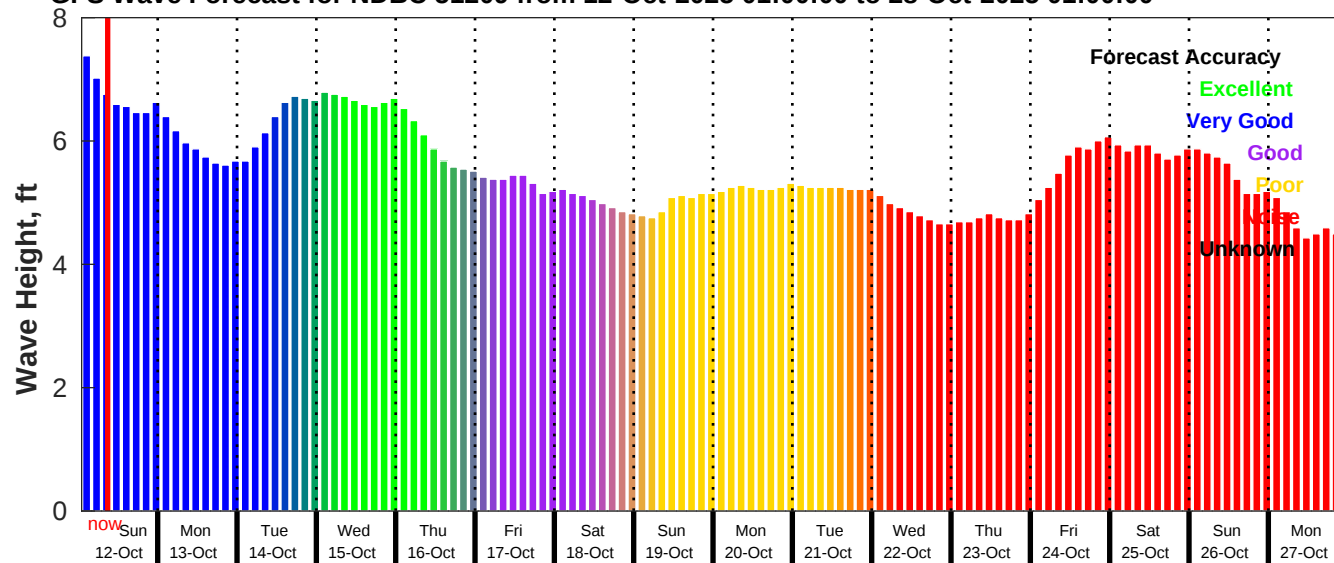
GFS Wave Forecast for NDBC 51209 from 12-Oct-2025 01:00:00 to 28-Oct-2025 01:00:00
