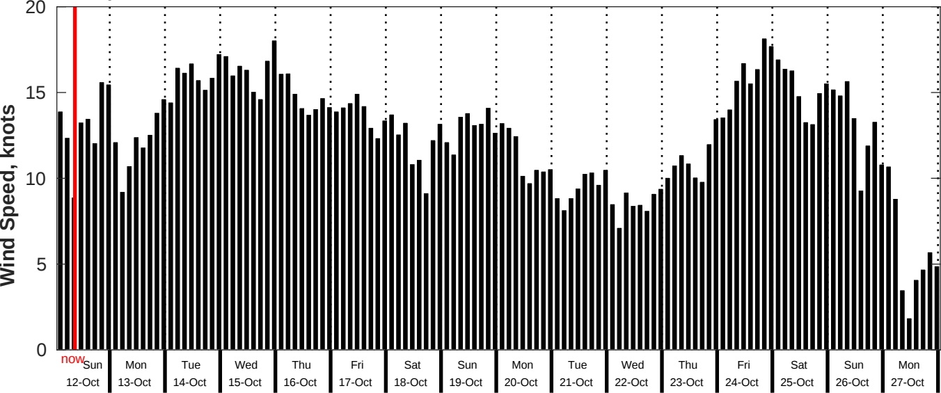
GFS Wind Speed Forecast for NDBC 51209 from 12-Oct-2025 01:00:00 to 28-Oct-2025 01:00:00
