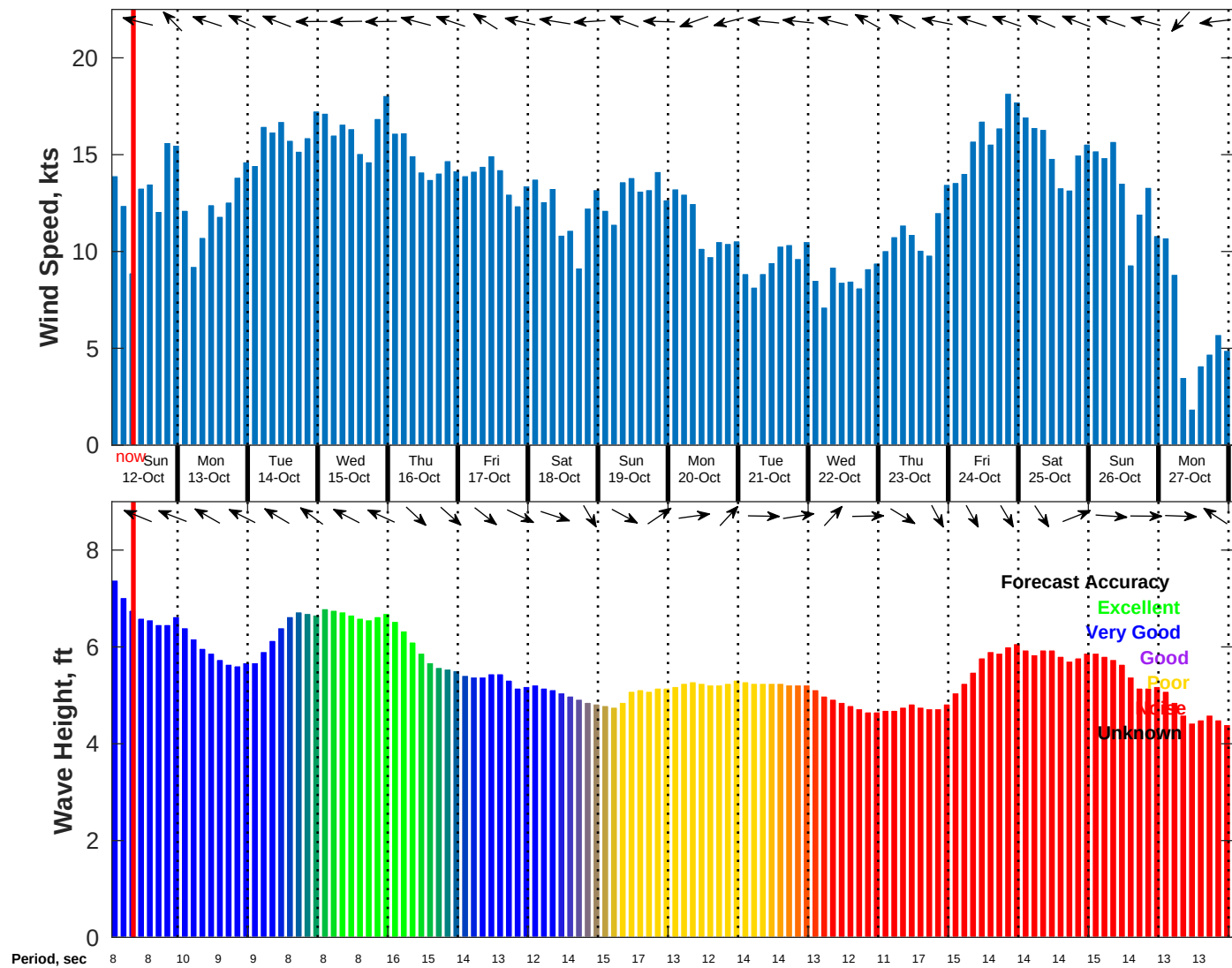
Wind & Wave Forecast for NDBC 51209 from 12-Oct-2025 01:00:00 to 28-Oct-2025 01:00:00
