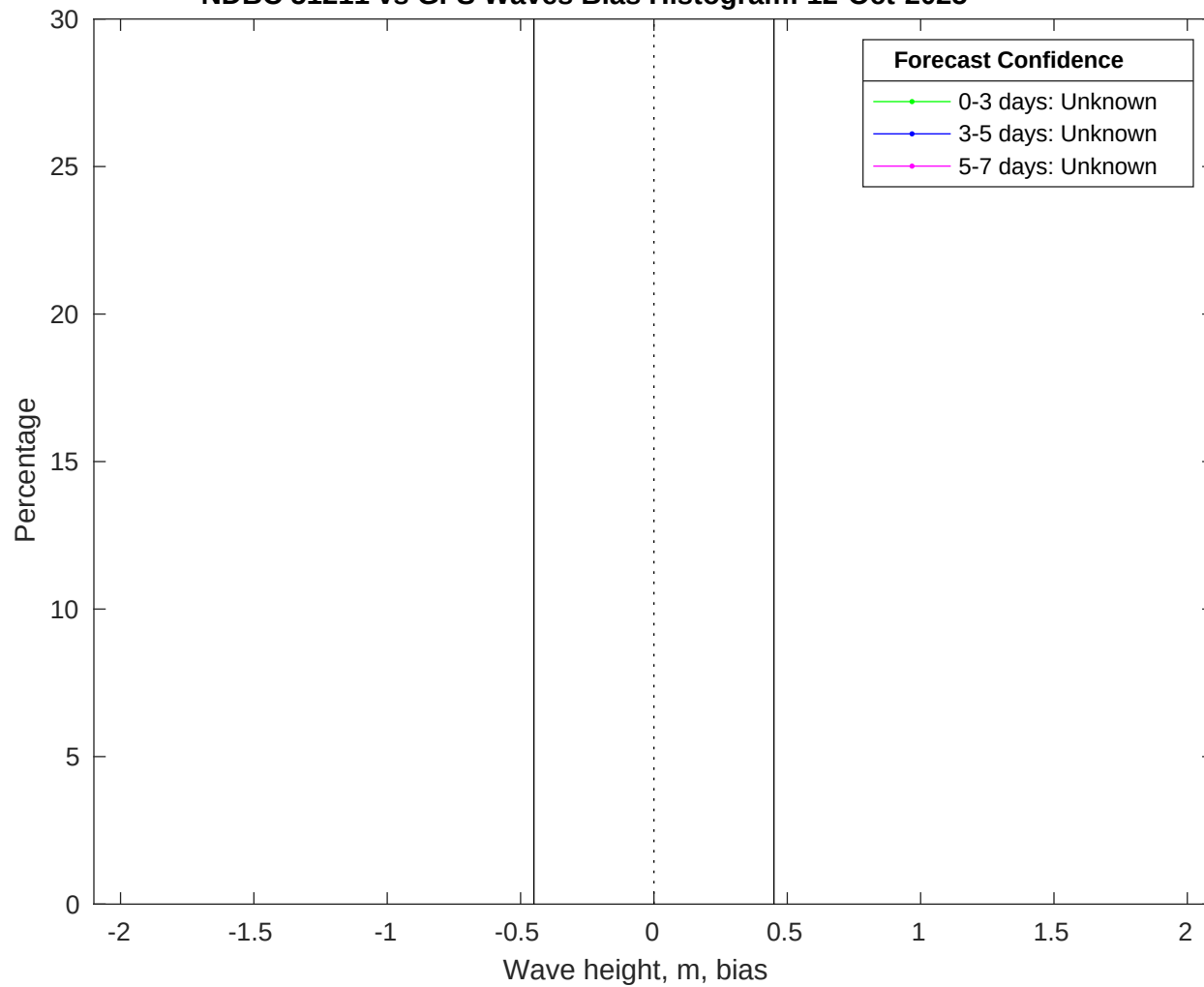
NDBC 51211 vs GFS Waves Bias Histogram: 12-Oct-2025
