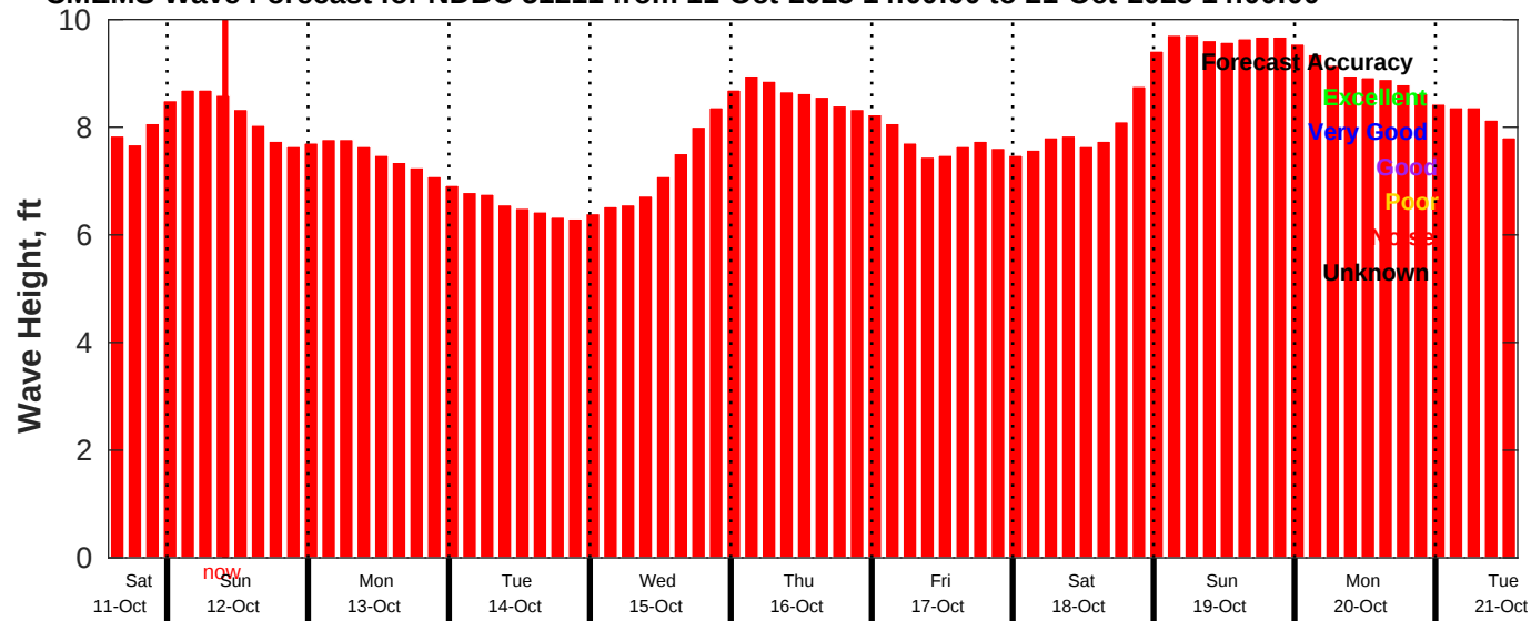
CMEMS Wave Forecast for NDBC 51211 from 11-Oct-2025 14:00:00 to 21-Oct-2025 14:00:00
