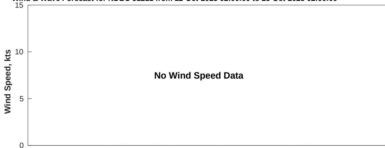
Wind & Wave Forecast for NDBC 51211 from 12-Oct-2025 02:00:00 to 28-Oct-2025 02:00:00
