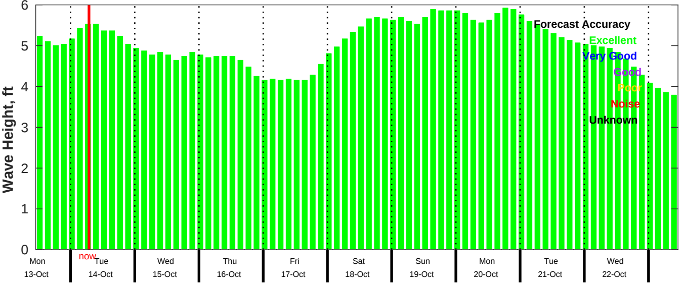
CMEMS Wave Forecast for NDBC 52211 from 12-Oct-2025 11:00:00 to 22-Oct-2025 11:00:00
