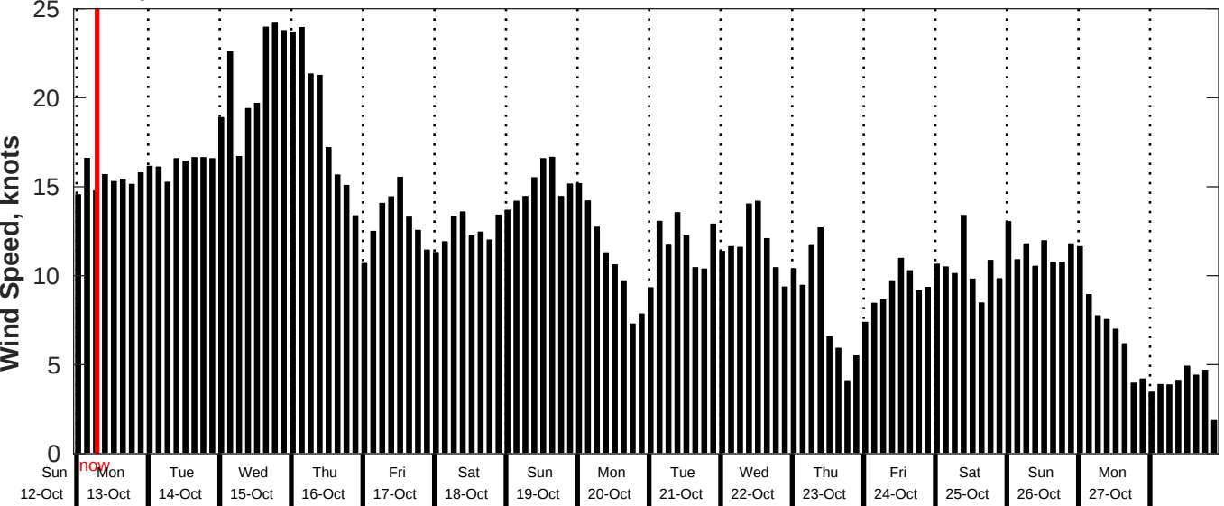
GFS Wind Speed Forecast for NDBC 52211 from 12-Oct-2025 23:00:00 to 28-Oct-2025 23:00:00
