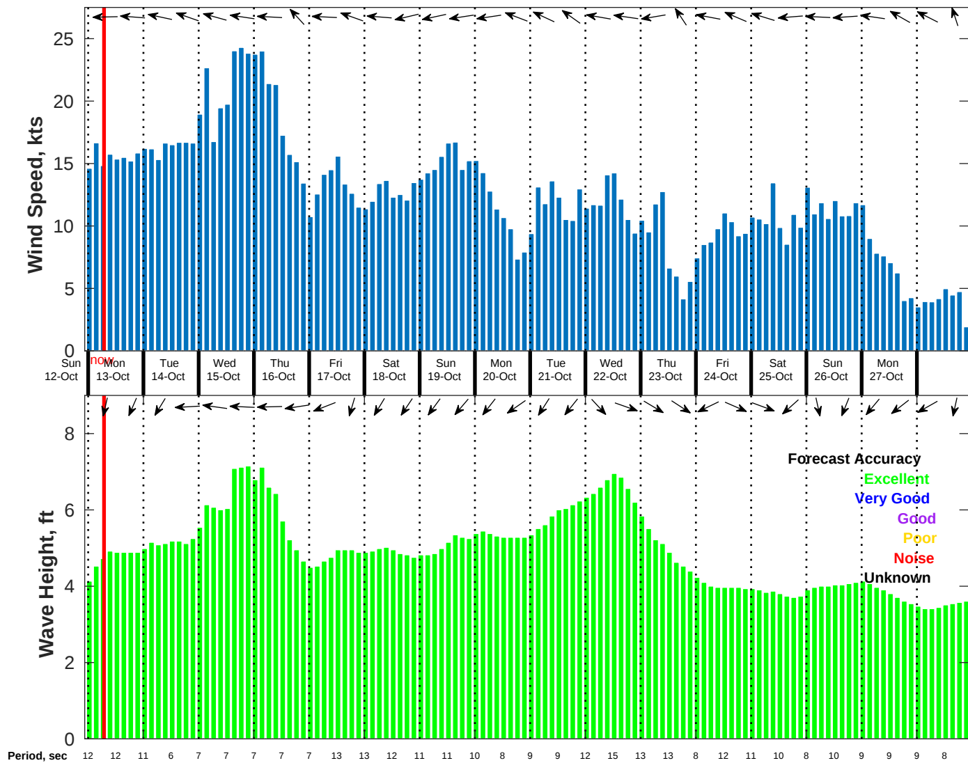
Wind & Wave Forecast for NDBC 52211 from 12-Oct-2025 23:00:00 to 28-Oct-2025 23:00:00
