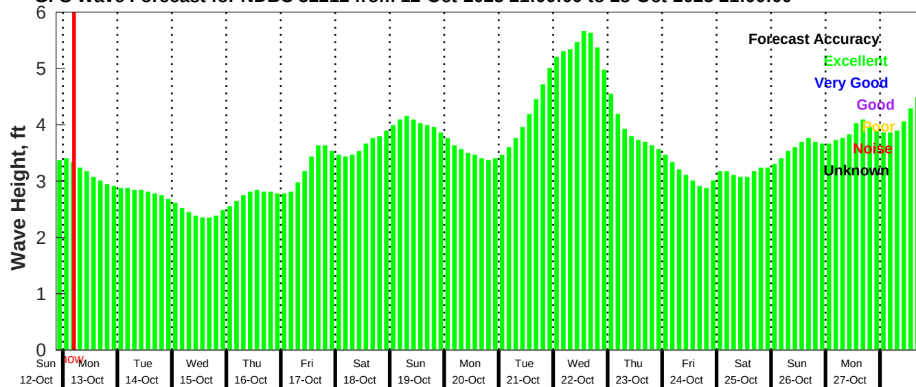
GFS Wave Forecast for NDBC 52212 from 12-Oct-2025 21:00:00 to 28-Oct-2025 21:00:00
