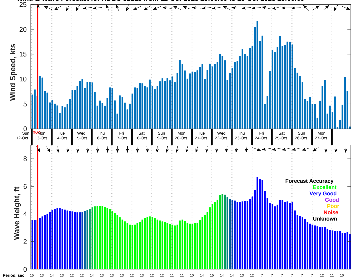
Wind & Wave Forecast for NDBC 52213 from 12-Oct-2025 23:00:00 to 28-Oct-2025 23:00:00
