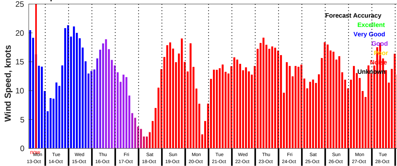
GFS Wind Speed Forecast for NDBC 41004 from 13-Oct-2025 07:00:00 to 29-Oct-2025 07:00:00
