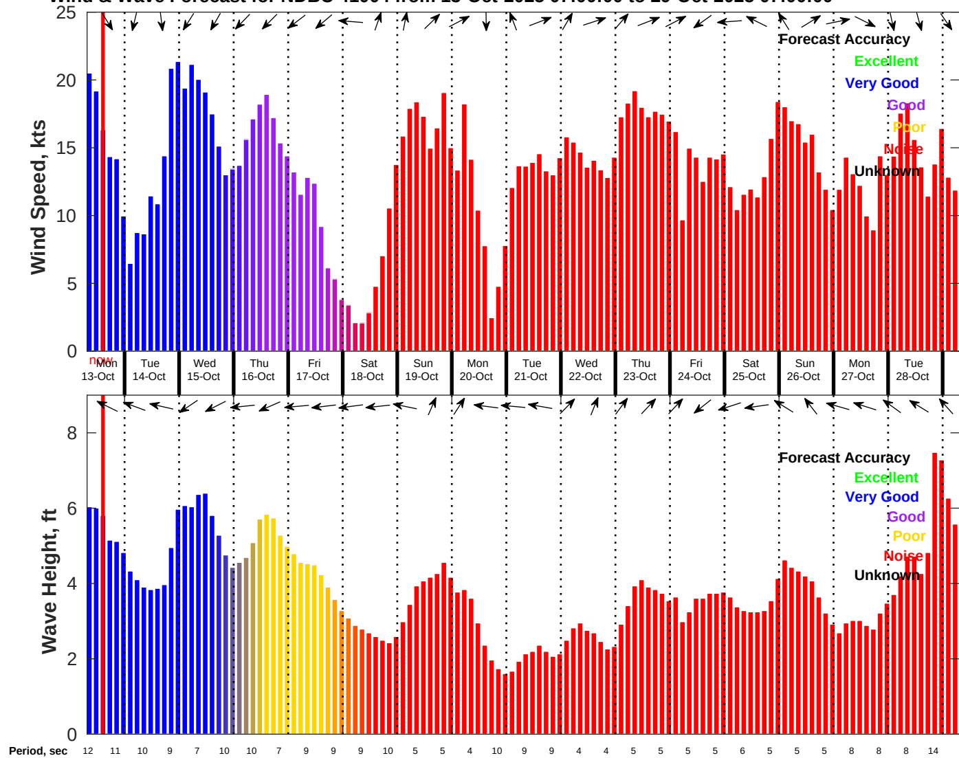
Wind & Wave Forecast for NDBC 41004 from 13-Oct-2025 07:00:00 to 29-Oct-2025 07:00:00
