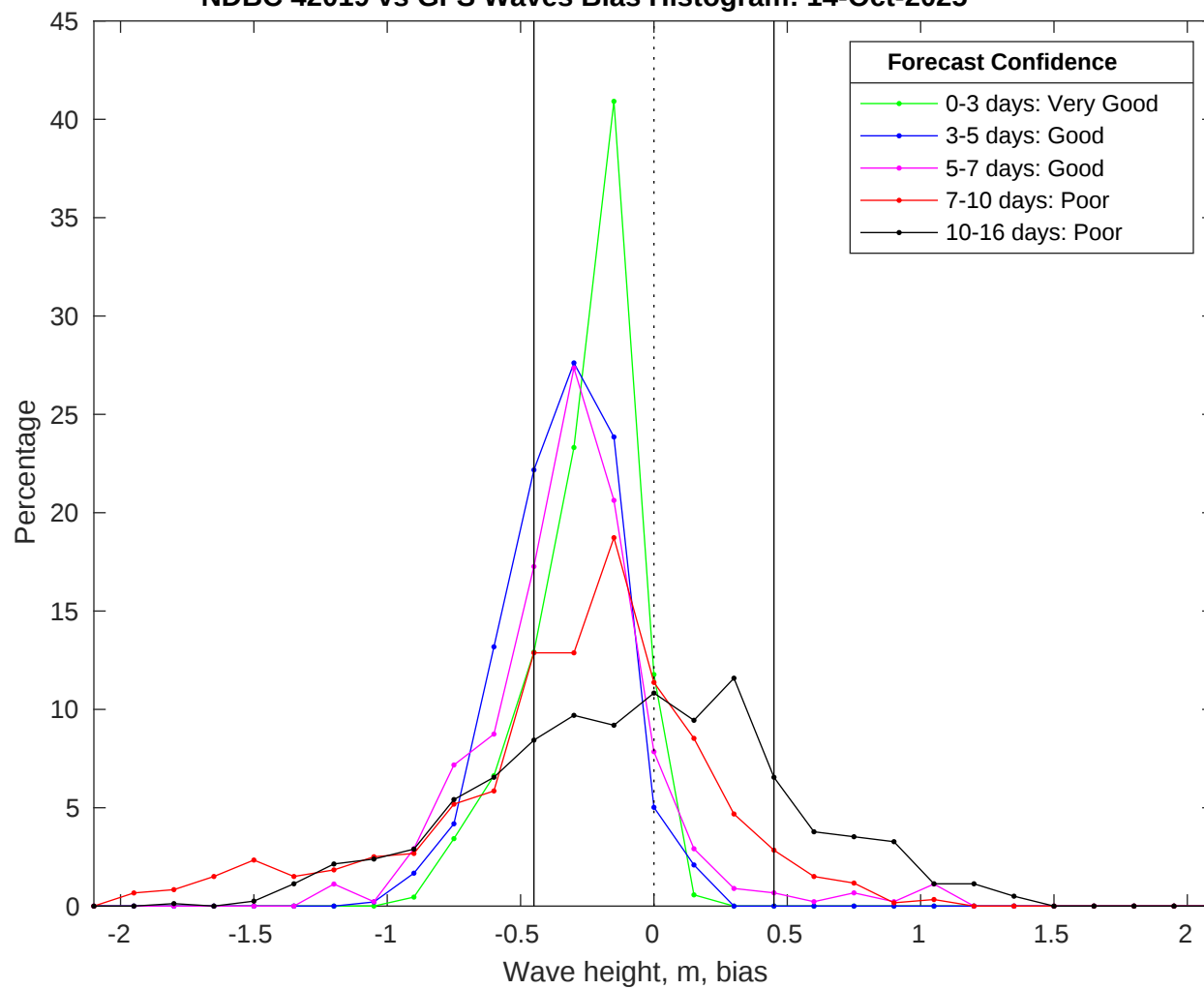
NDBC 42019 vs GFS Waves Bias Histogram: 14-Oct-2025
