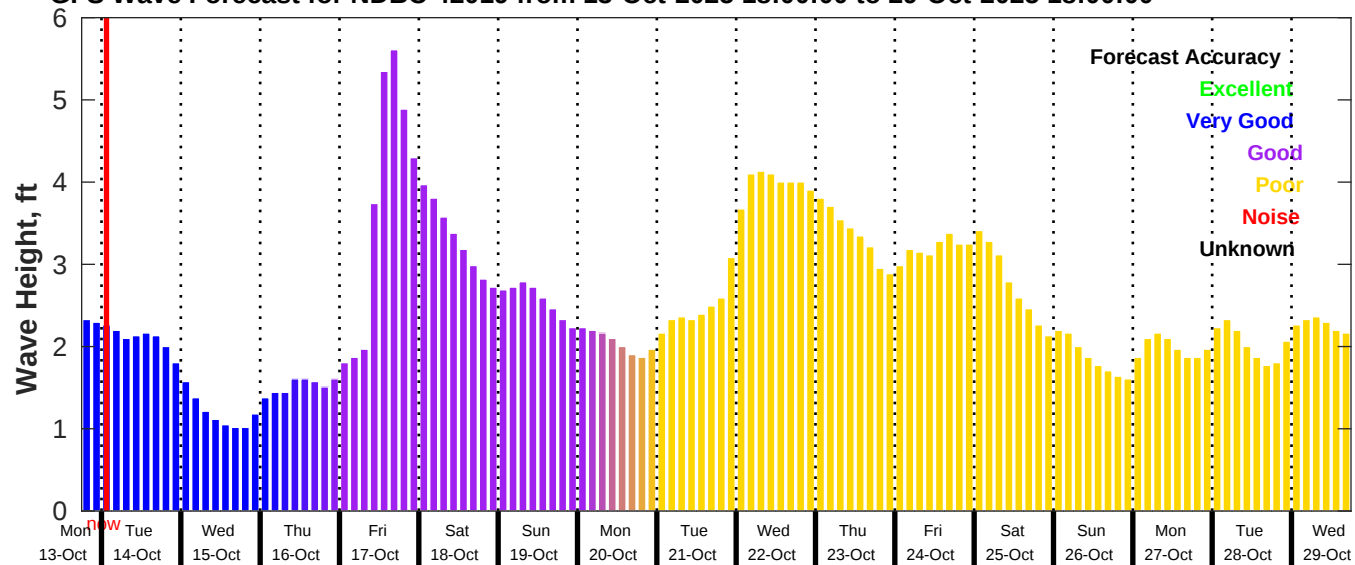
GFS Wave Forecast for NDBC 42019 from 13-Oct-2025 18:00:00 to 29-Oct-2025 18:00:00
