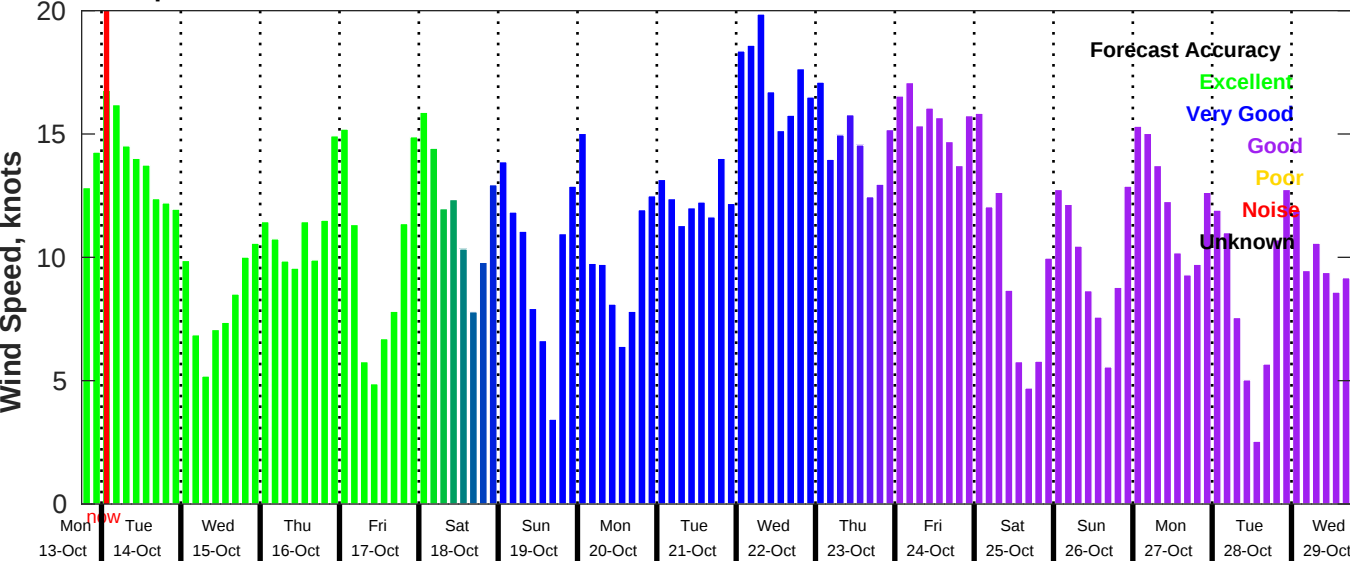
GFS Wind Speed Forecast for NDBC 42020 from 13-Oct-2025 18:00:00 to 29-Oct-2025 18:00:00
