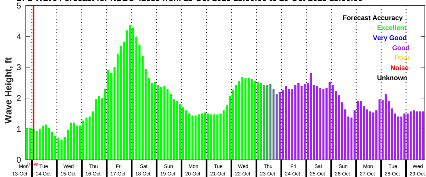
GFS Wave Forecast for NDBC 42035 from 13-Oct-2025 18:00:00 to 29-Oct-2025 18:00:00
