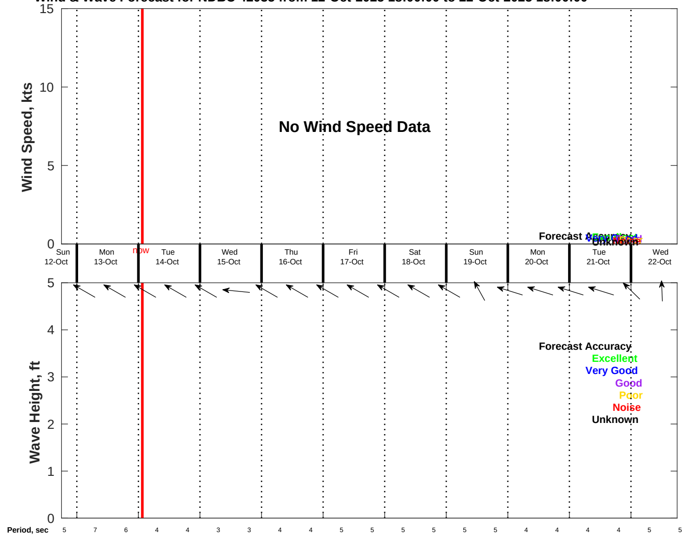
Wind & Wave Forecast for NDBC 42035 from 12-Oct-2025 18:00:00 to 22-Oct-2025 18:00:00
