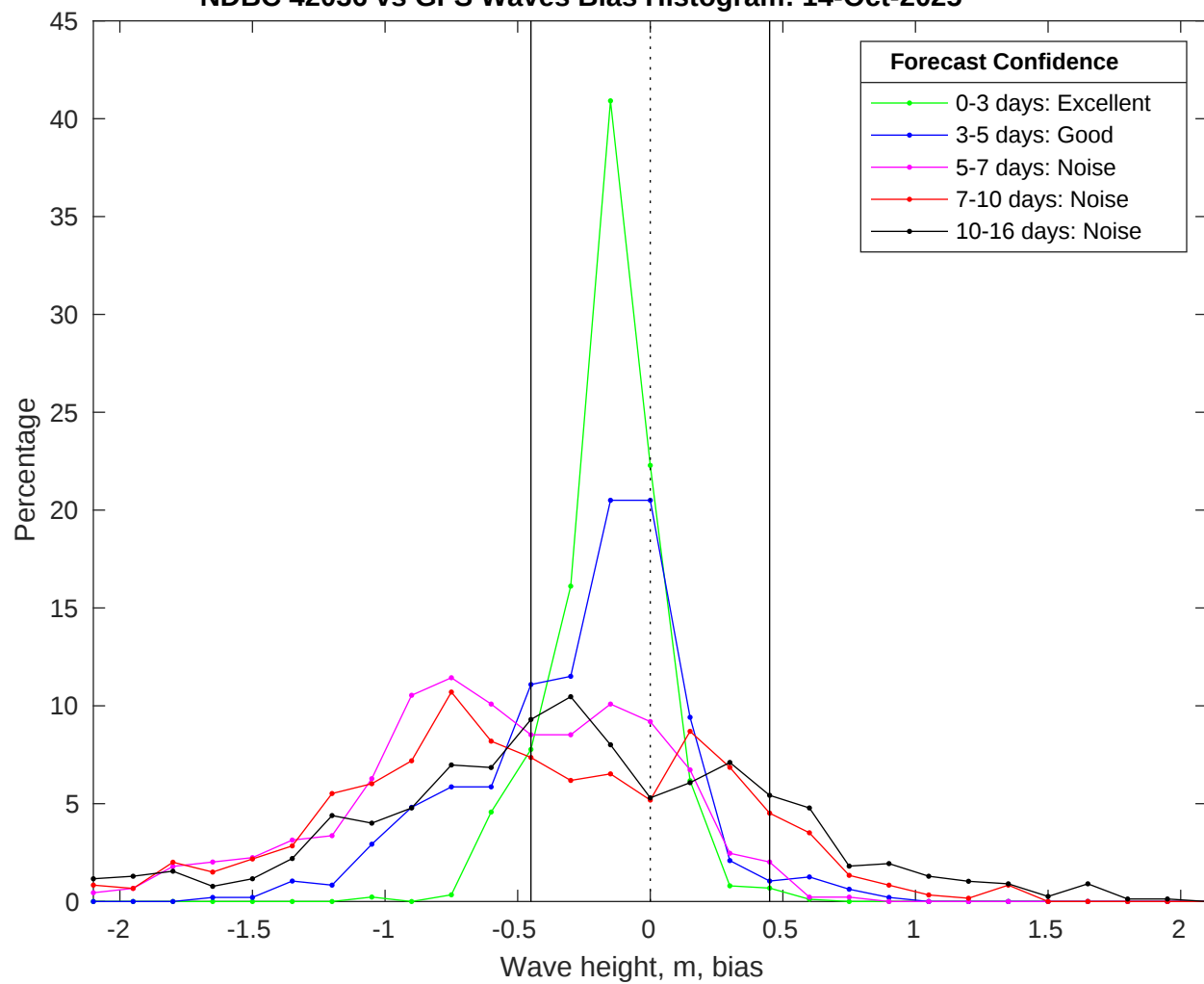
NDBC 42036 vs GFS Waves Bias Histogram: 14-Oct-2025
