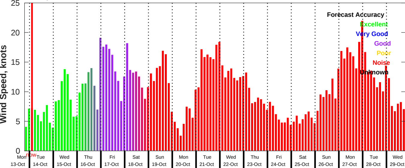
GFS Wind Speed Forecast for NDBC 42036 from 13-Oct-2025 19:00:00 to 29-Oct-2025 19:00:00
