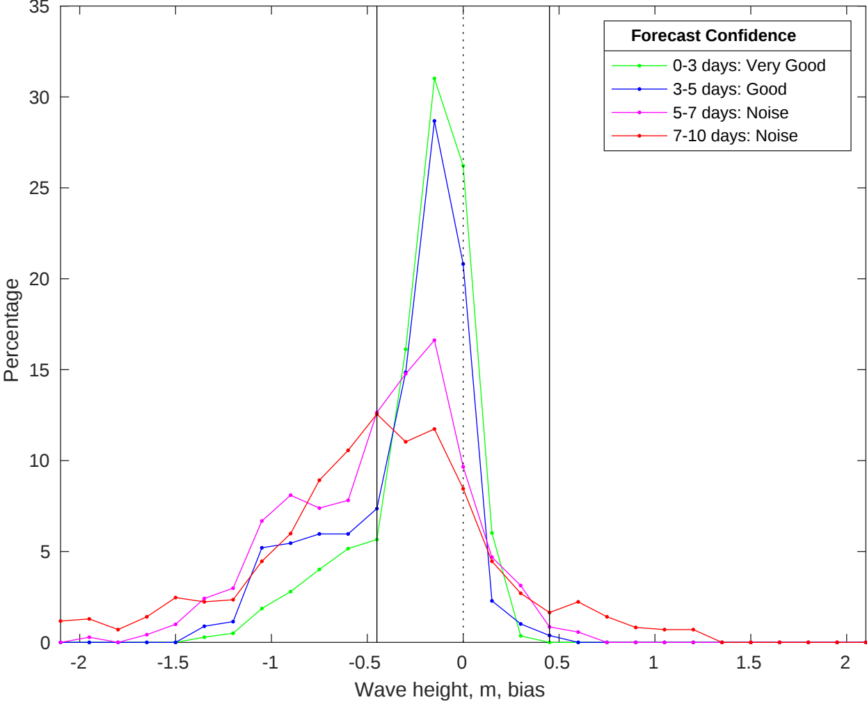
NDBC 42040 vs CMEMS Waves Bias Histogram: 14-Oct-2025
