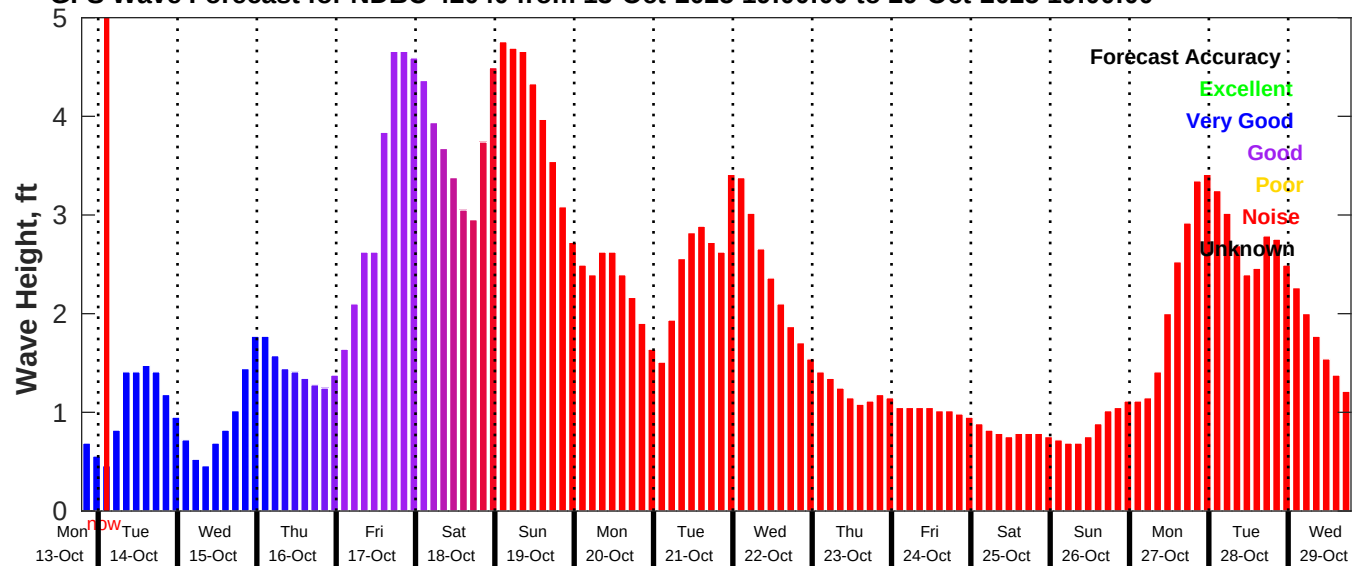
GFS Wave Forecast for NDBC 42040 from 13-Oct-2025 19:00:00 to 29-Oct-2025 19:00:00
