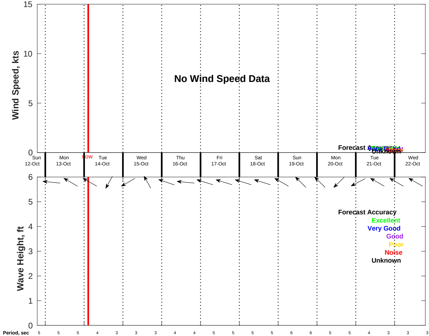
Wind & Wave Forecast for NDBC 42040 from 12-Oct-2025 19:00:00 to 22-Oct-2025 19:00:00
