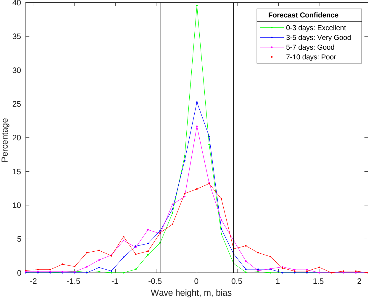
NDBC 44008 vs CMEMS Waves Bias Histogram: 14-Oct-2025
