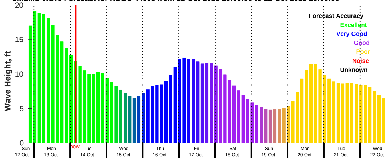
CMEMS Wave Forecast for NDBC 44008 from 12-Oct-2025 20:00:00 to 22-Oct-2025 20:00:00
