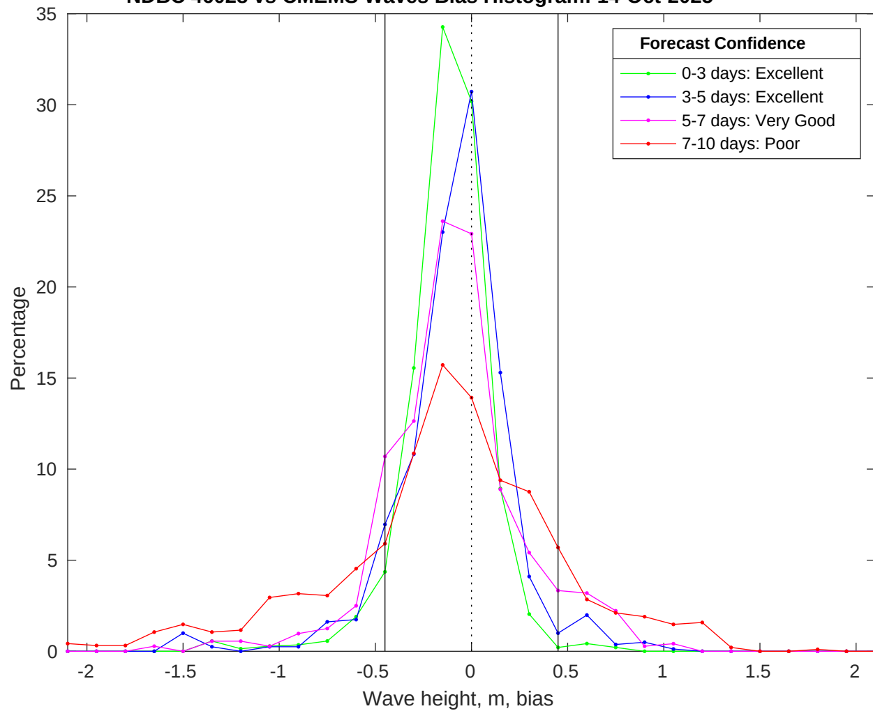
NDBC 46028 vs CMEMS Waves Bias Histogram: 14-Oct-2025
