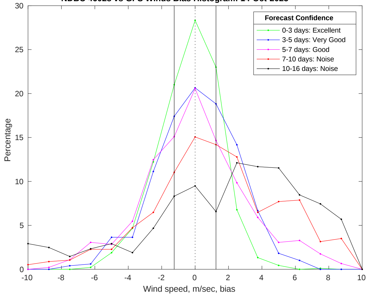
NDBC 46028 vs GFS Winds Bias Histogram: 14-Oct-2025
