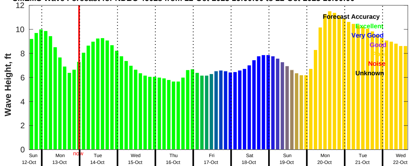
CMEMS Wave Forecast for NDBC 46028 from 12-Oct-2025 16:00:00 to 22-Oct-2025 16:00:00
