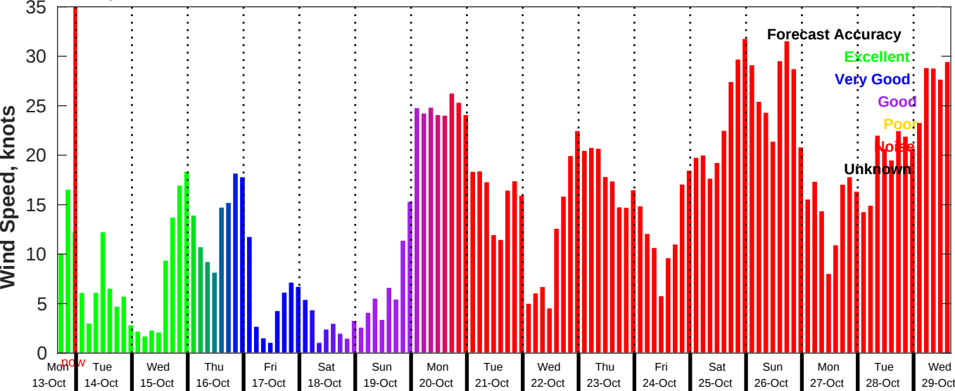
GFS Wind Speed Forecast for NDBC 46028 from 13-Oct-2025 16:00:00 to 29-Oct-2025 16:00:00
