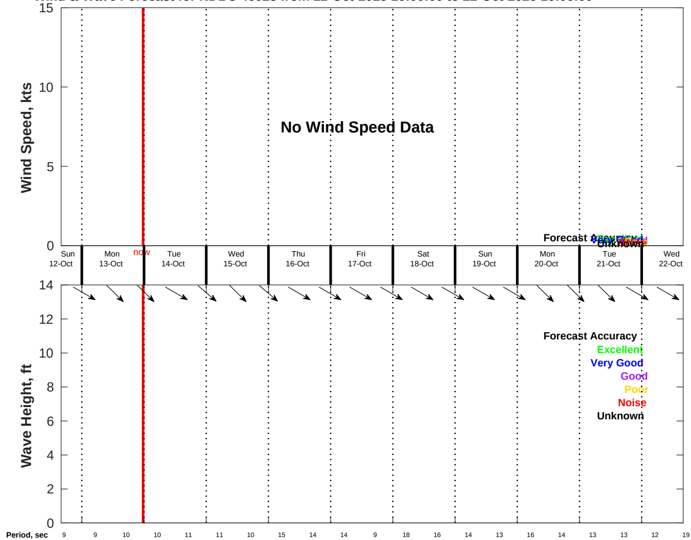
Wind & Wave Forecast for NDBC 46028 from 12-Oct-2025 16:00:00 to 22-Oct-2025 16:00:00
