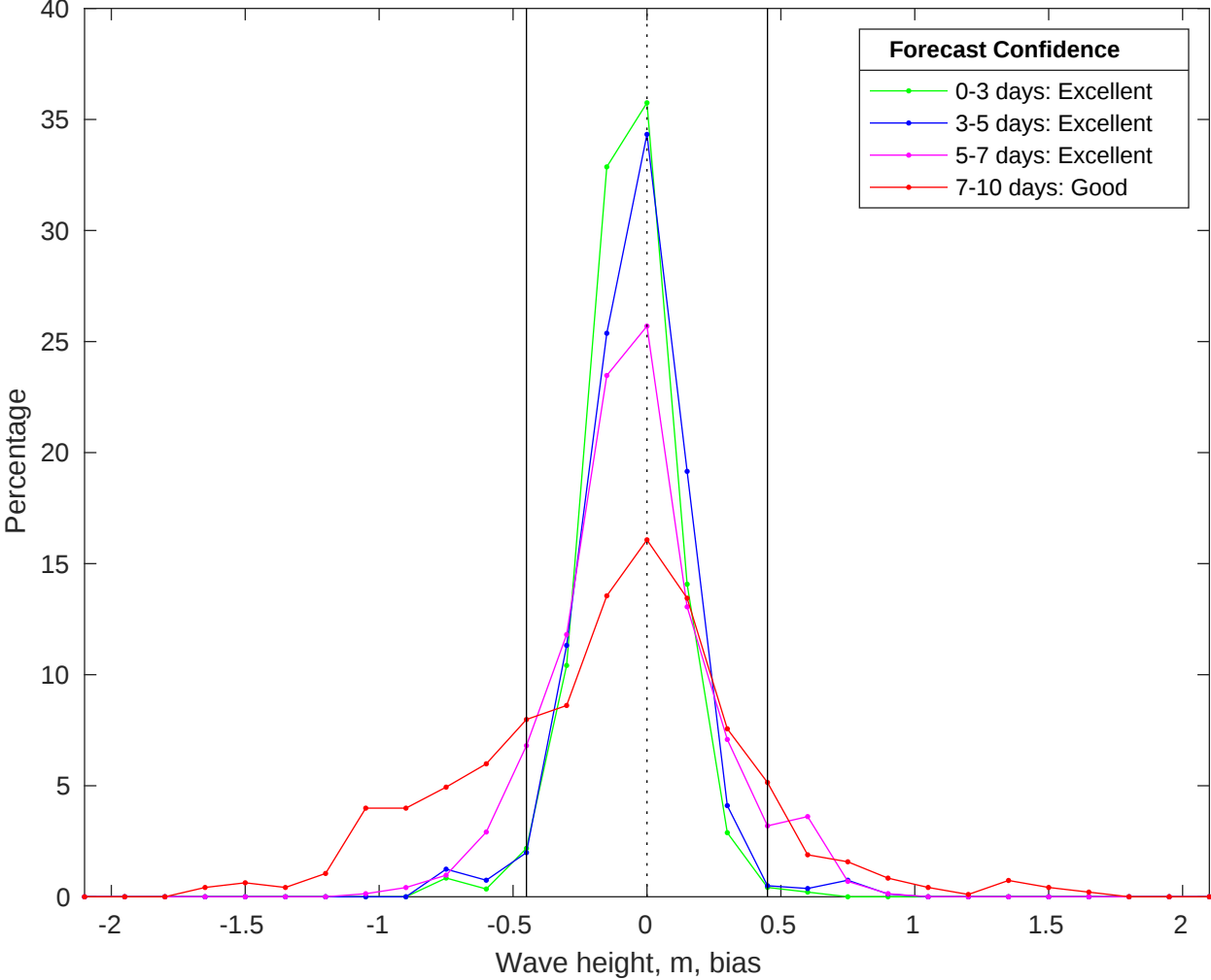
NDBC 46054 vs CMEMS Waves Bias Histogram: 14-Oct-2025
