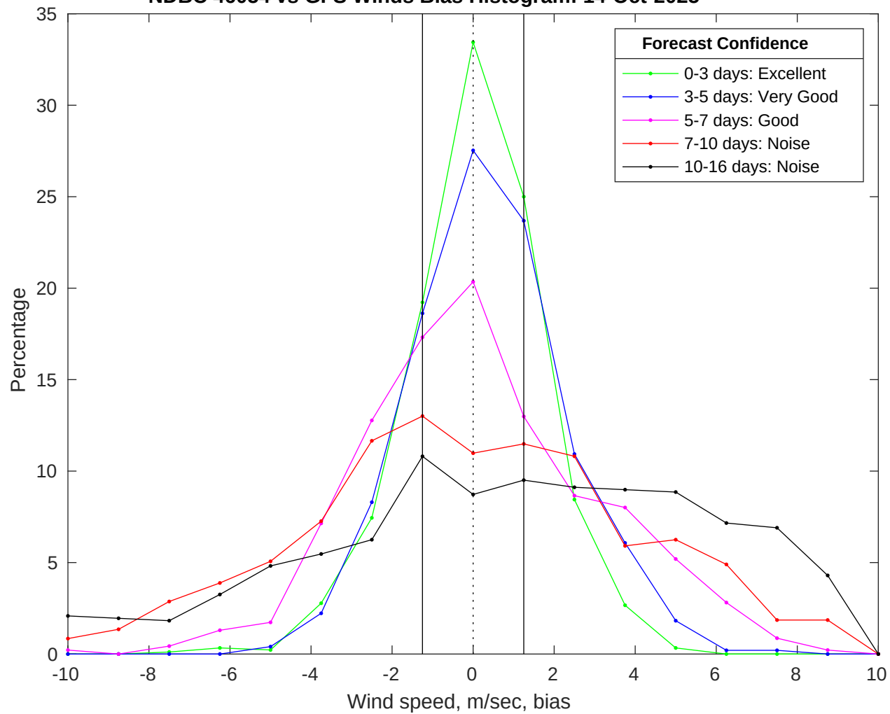
NDBC 46054 vs GFS Winds Bias Histogram: 14-Oct-2025
