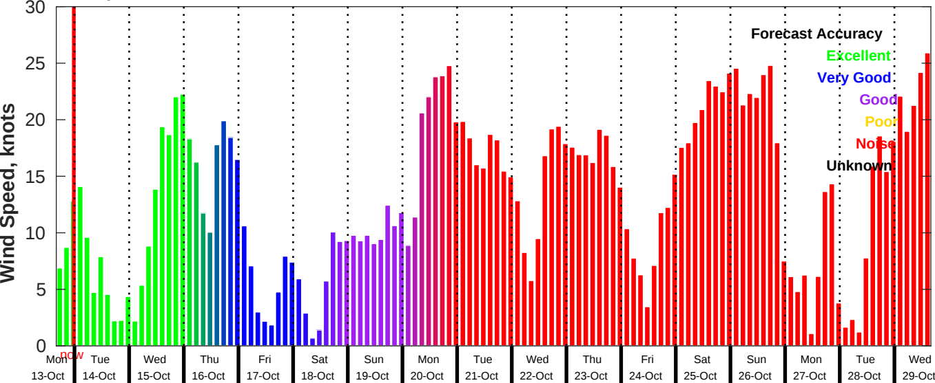
GFS Wind Speed Forecast for NDBC 46054 from 13-Oct-2025 16:00:00 to 29-Oct-2025 16:00:00
