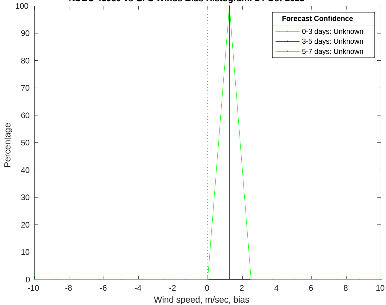
NDBC 46059 vs GFS Winds Bias Histogram: 14-Oct-2025
