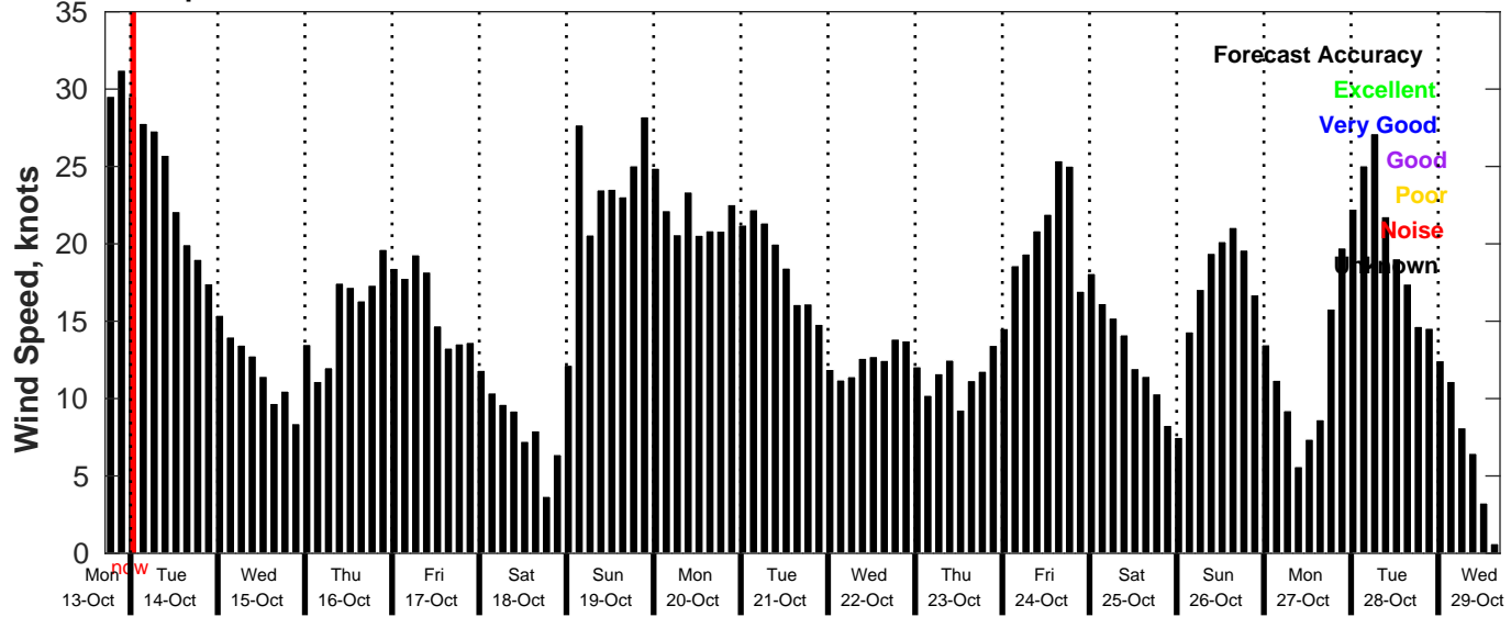
GFS Wind Speed Forecast for NDBC 46059 from 13-Oct-2025 17:00:00 to 29-Oct-2025 17:00:00
