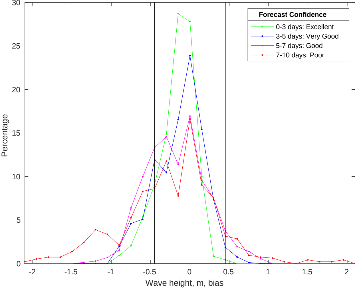
NDBC 46069 vs CMEMS Waves Bias Histogram: 14-Oct-2025
