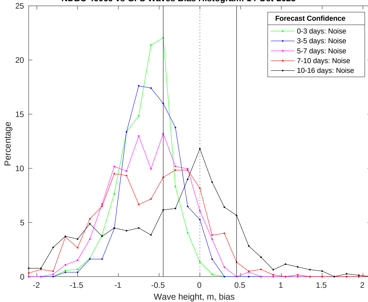
NDBC 46069 vs GFS Waves Bias Histogram: 14-Oct-2025
