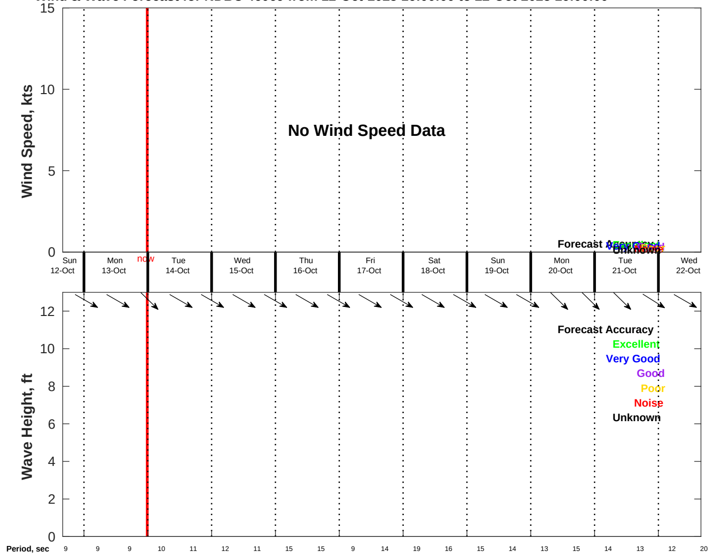
Wind & Wave Forecast for NDBC 46069 from 12-Oct-2025 16:00:00 to 22-Oct-2025 16:00:00
