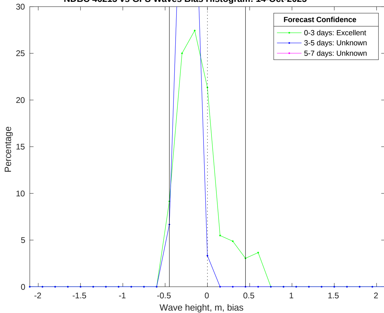
NDBC 46215 vs GFS Waves Bias Histogram: 14-Oct-2025
